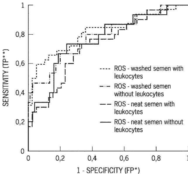
Receiver operating characteristic curves showing the area under the curve in male factor infertility patients and fertile men using reactive oxygen species level on neat and washed semen with or without leukocytes. *FP indicates false positive; **TP, true positive.
